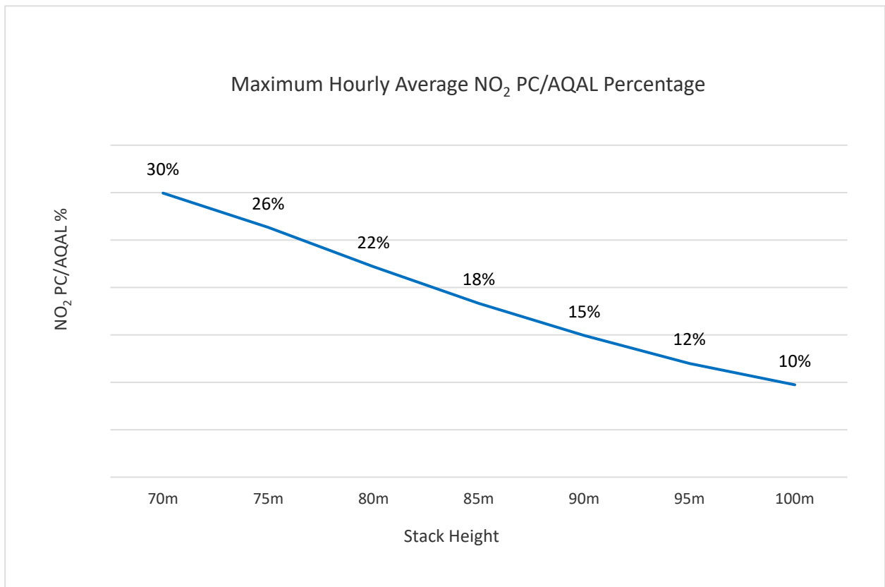
Plate 8B.2: Stack Height Determination (Hydrogen Firing)
